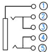
MATE PLUG
